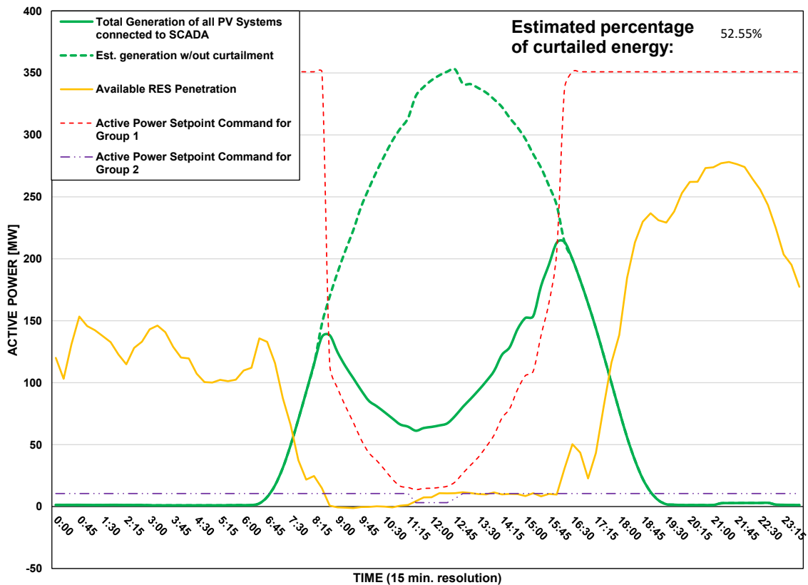
Scada PVs Generation on 23/08/2026 (curtailment time: 08:30 - 16:00)
