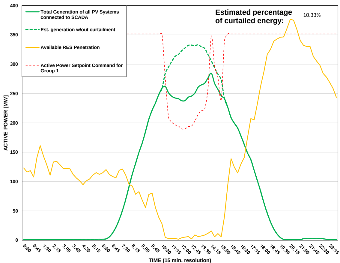
Scada PVs Generation on 11/08/2026 (curtailment time: 10:45 - 15:00)
