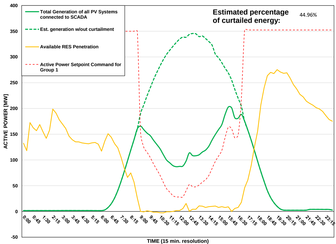
Scada PVs Generation on 01/08/2026 (curtailment time: 09:00 - 16:45)
