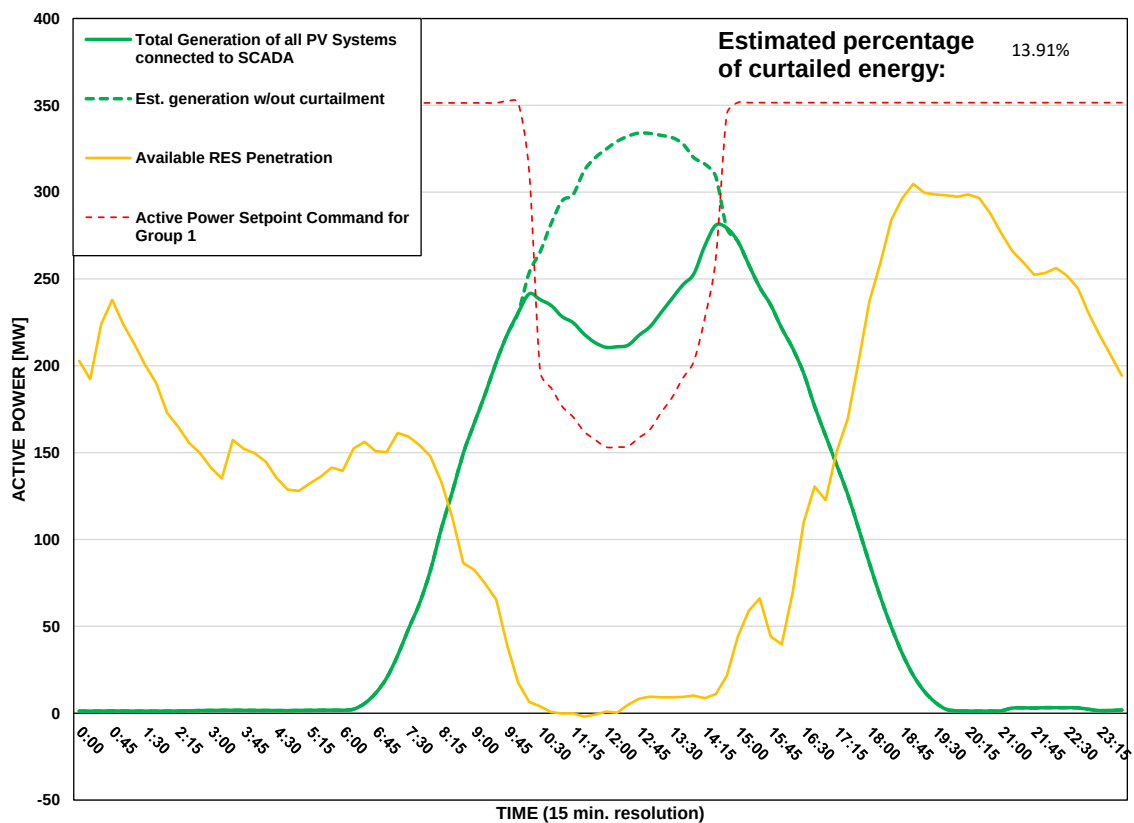
Scada PVs Generation on 07/08/2026 (curtailment time: 10:15 - 14:30)
