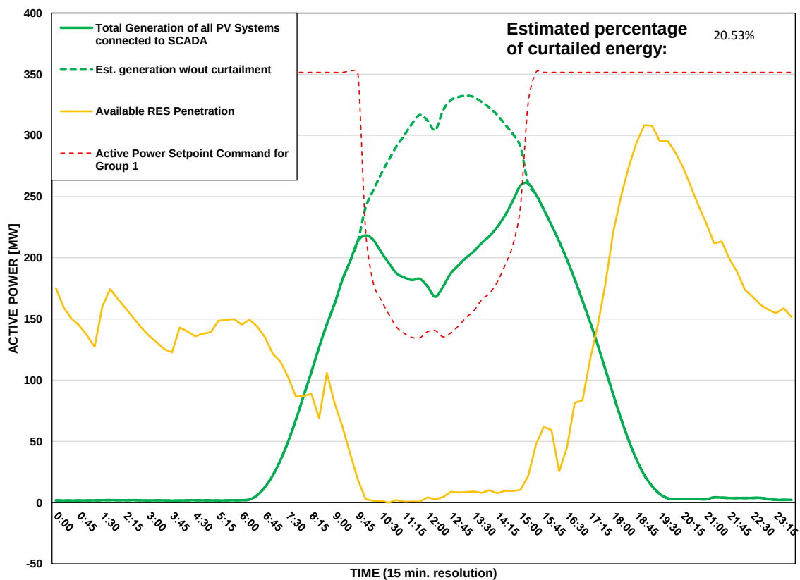
Scada PVs Generation on 08/08/2026 (curtailment time: 10:00 - 15:00)
