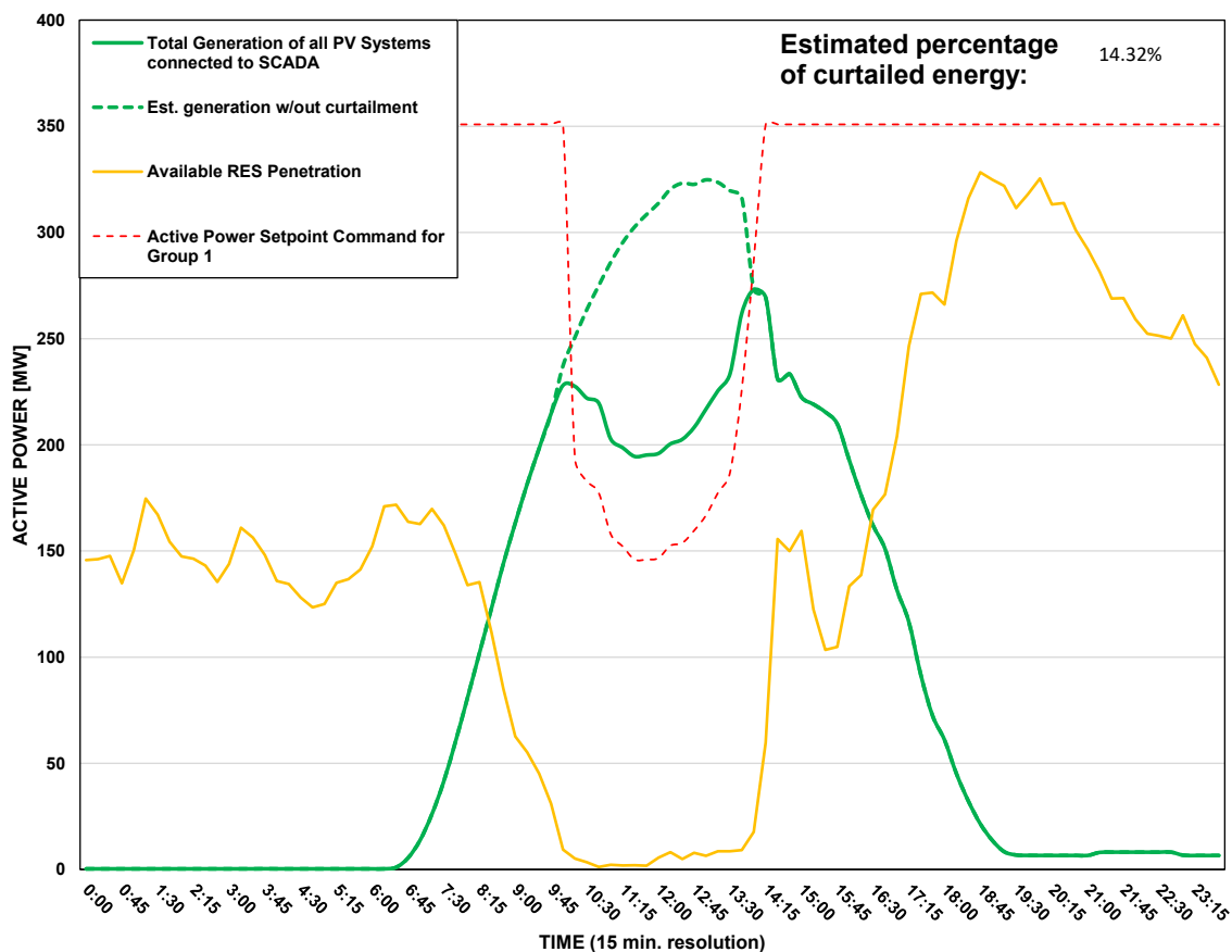
Scada PVs Generation on 28/08/2026 (curtailment time: 10:00 - 13:45)
