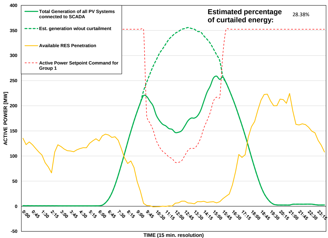
Scada PVs Generation on 03/08/2026 (curtailment time: 09:30 - 15:30)
