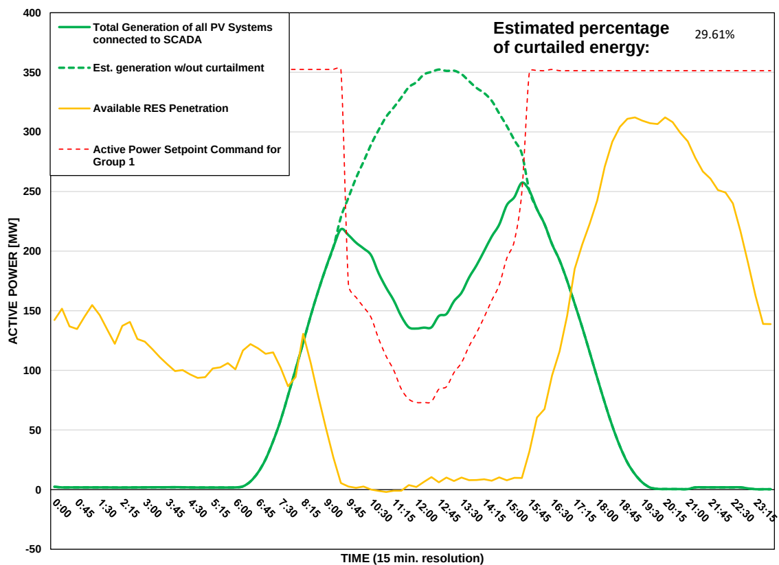
Scada PVs Generation on 04/08/2026 (curtailment time: 09:30 - 15:30)
