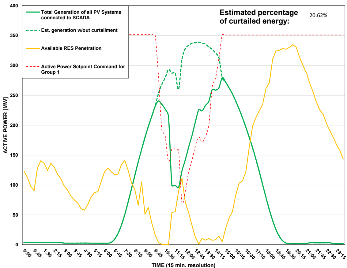
Scada PVs Generation on 21/08/2026 (curtailment time: 10:00 - 14:30)
