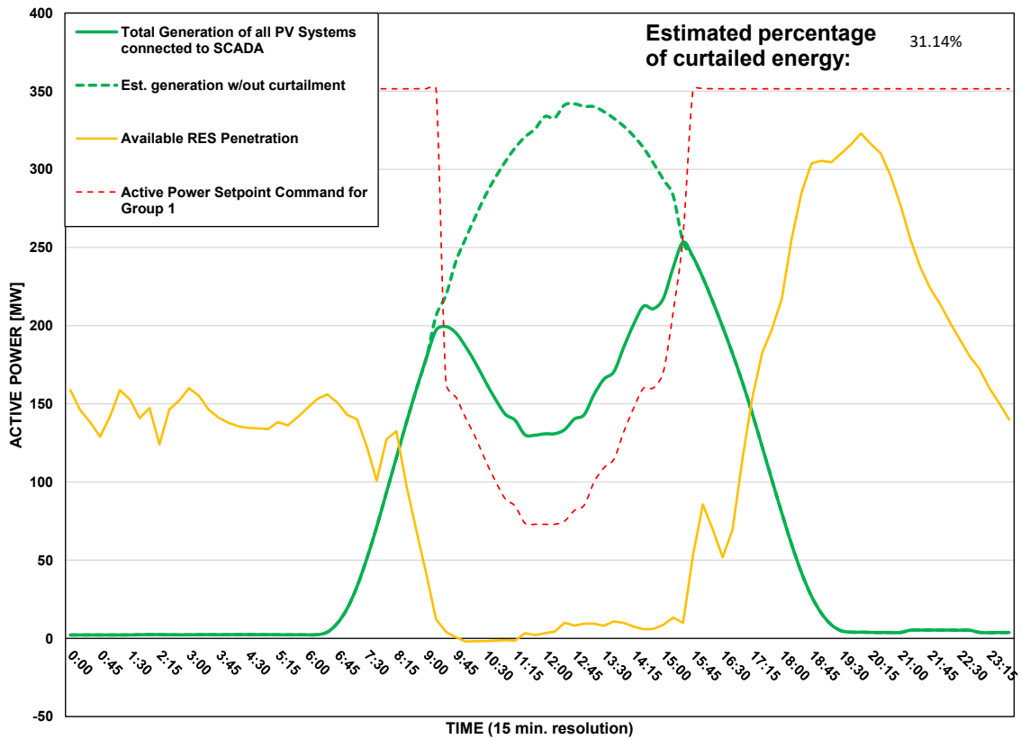
Scada PVs Generation on 20/08/2026 (curtailment time: 09:15 - 15:15)
