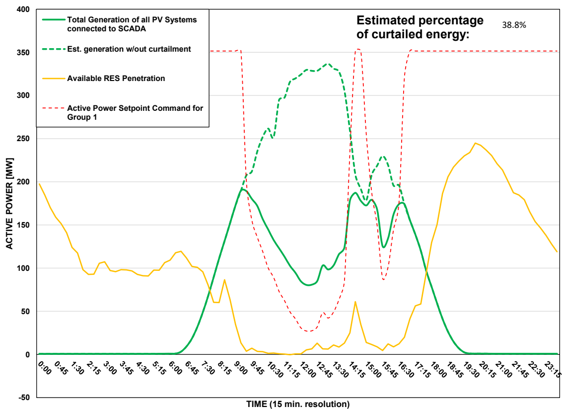
Scada PVs Generation on 18/08/2026 (curtailment time: 09:15 - 16:30)
