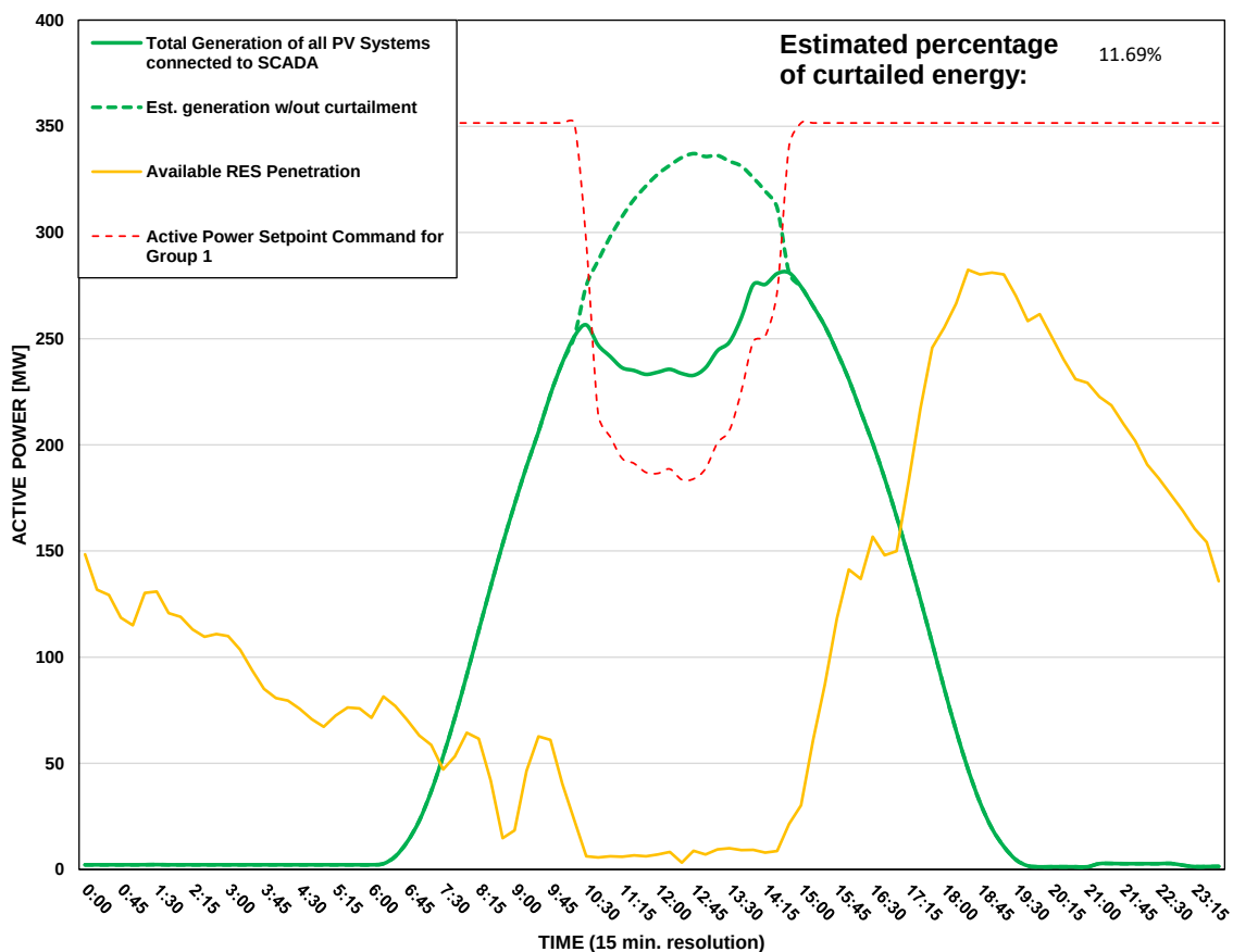
Scada PVs Generation on 10/08/2026 (curtailment time: 10:30 - 14:30)
