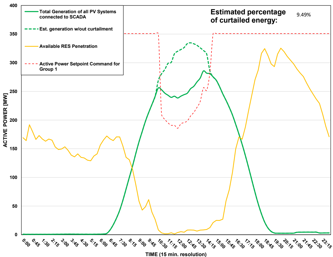
Scada PVs Generation on 25/08/2026 (curtailment time: 10:30 - 14:15)
