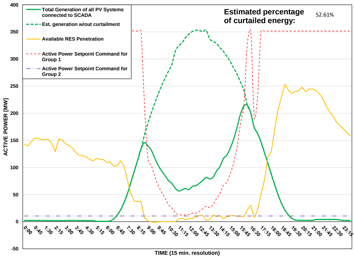
Scada PVs Generation on 09/08/2026 (curtailment time: 08:45 - 16:00)
