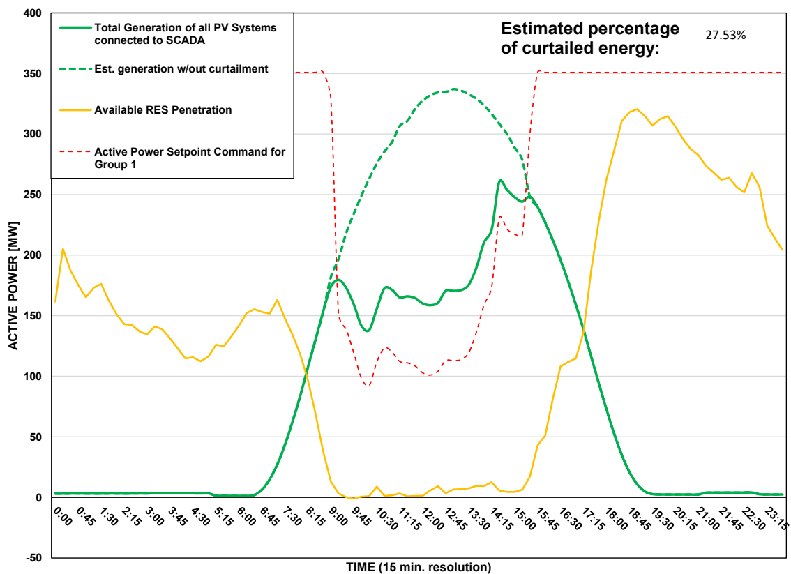
Scada PVs Generation on 26/08/2026 (curtailment time: 09:00 - 15:15)
