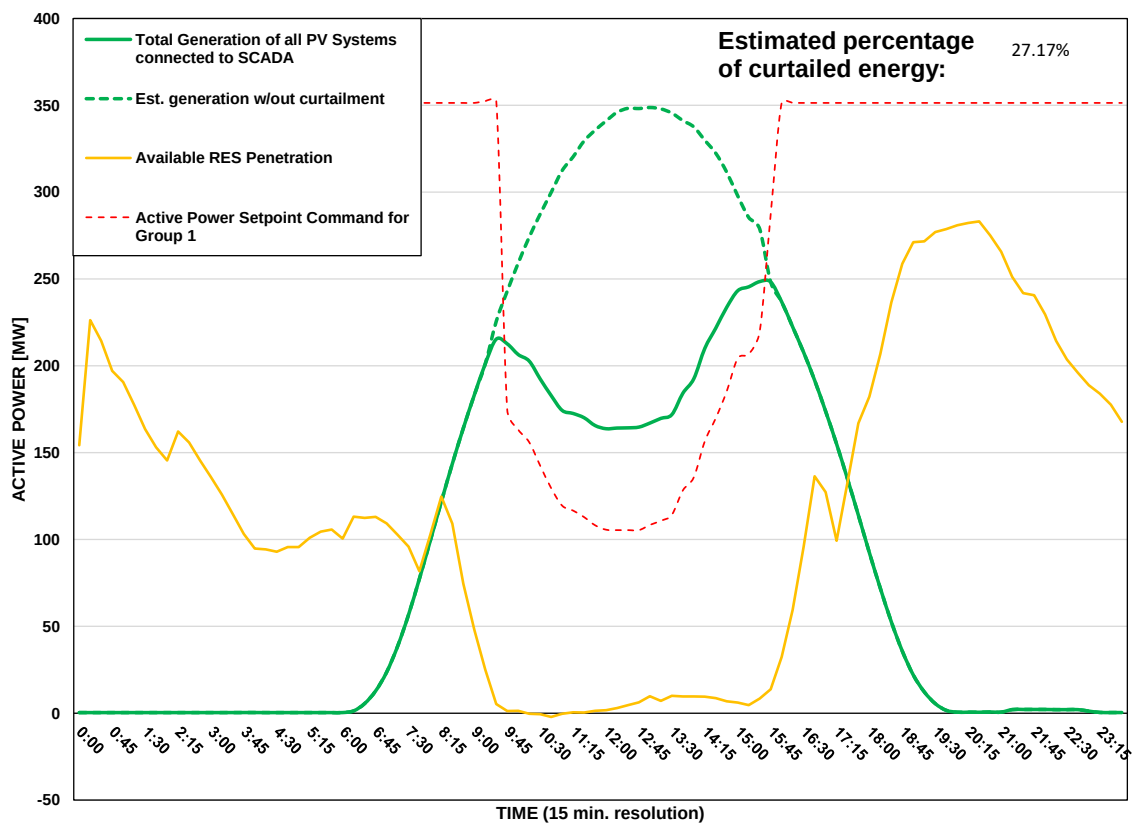
Scada PVs Generation on 05/08/2026 (curtailment time: 09:30 - 15:30)
