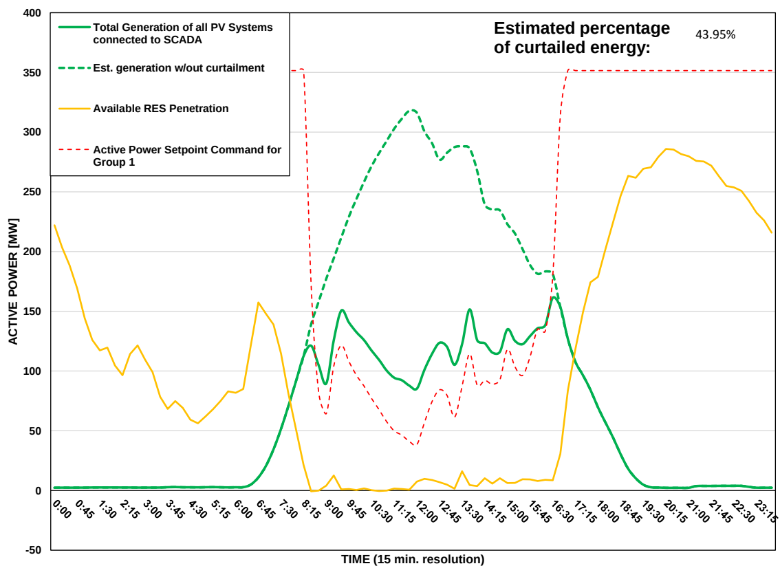
Scada PVs Generation on 15/08/2026 (curtailment time: 08:30 - 16:30)
