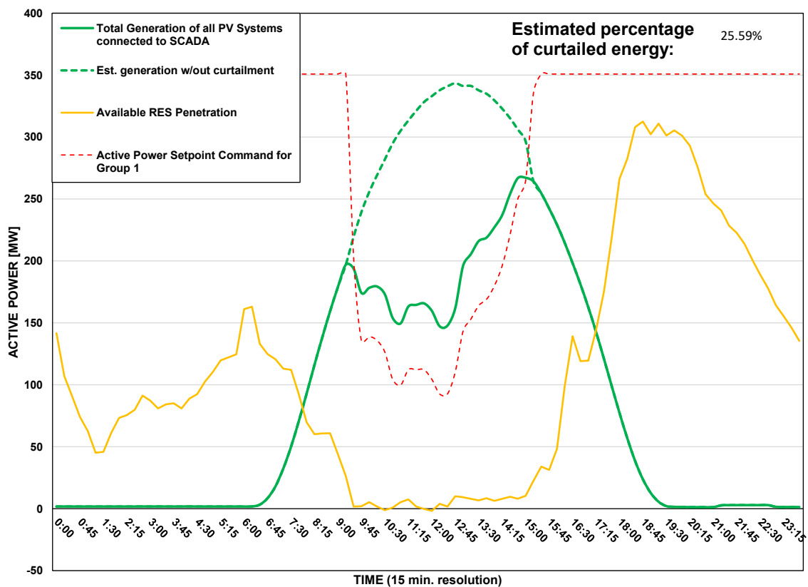
Scada PVs Generation on 22/08/2026 (curtailment time: 09:30 - 15:00)
