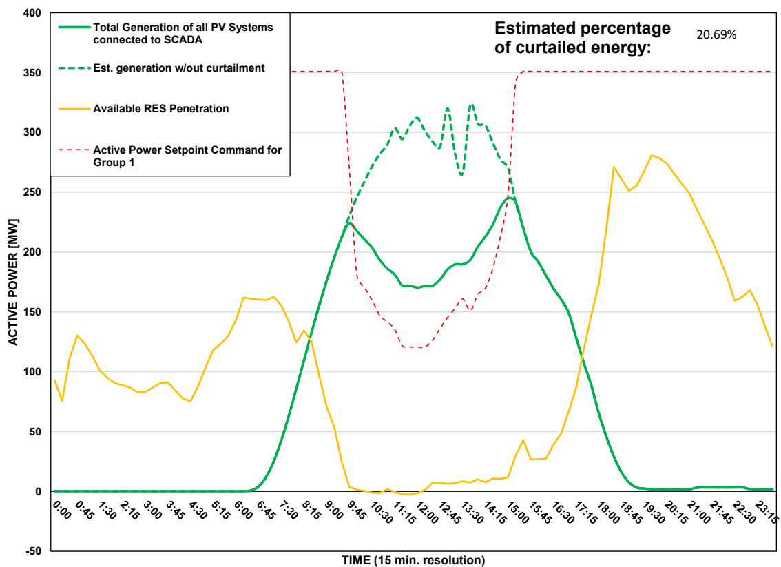
Scada PVs Generation on 31/08/2026 (curtailment time: 09:45 - 15:00)
