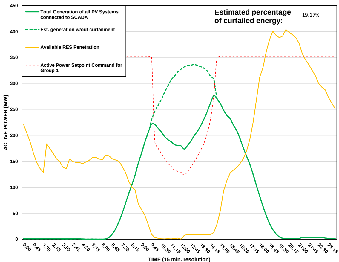
Scada PVs Generation on 12/08/2026 (curtailment time: 09:45 - 14:30)
