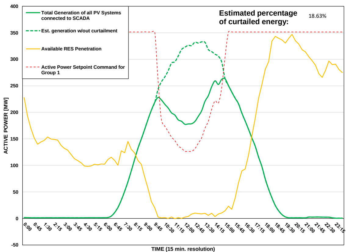
Scada PVs Generation on 13/08/2026 (curtailment time: 10:00 - 14:45)
