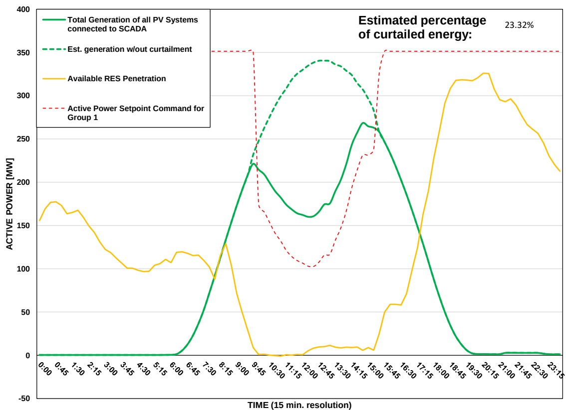
Scada PVs Generation on 06/08/2026 (curtailment time: 09:45 - 15:15)
