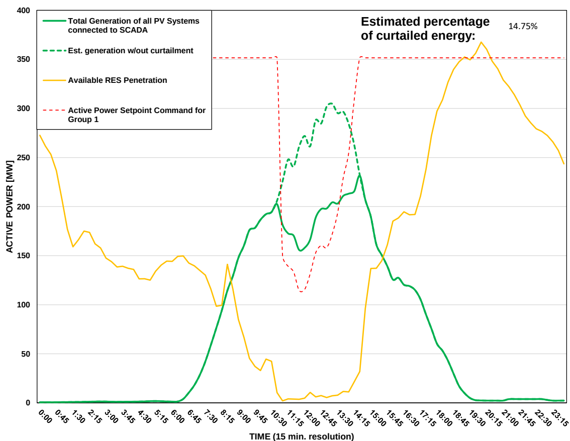
Scada PVs Generation on 14/08/2026 (curtailment time: 10:45 - 14:15)
