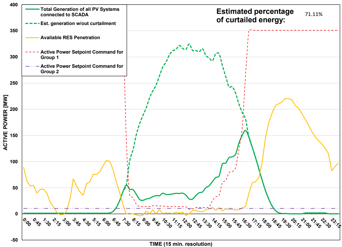
Scada PVs Generation on 30/08/2026 (curtailment time: 08:00 - 16:45)
