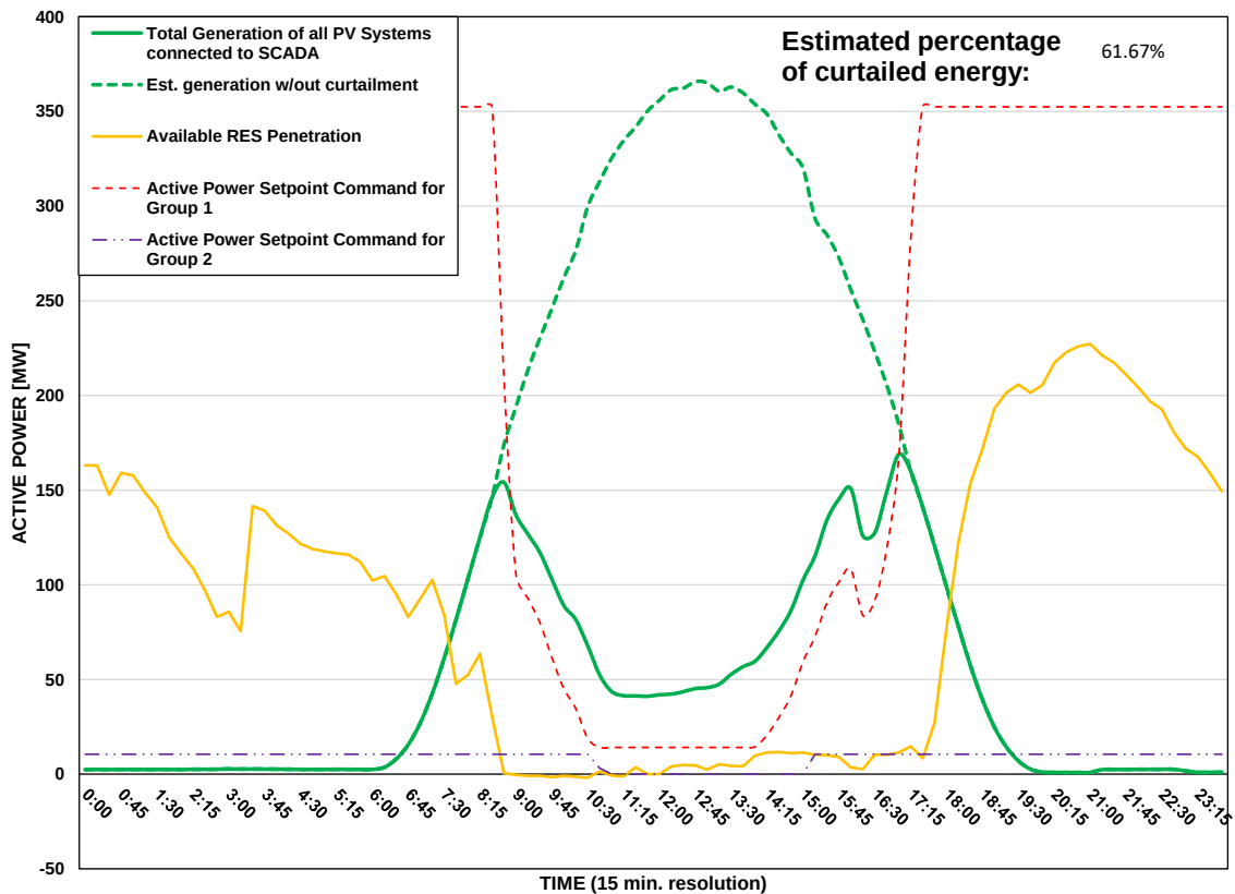
Scada PVs Generation on 02/08/2026 (curtailment time: 08:45 - 17:00)
