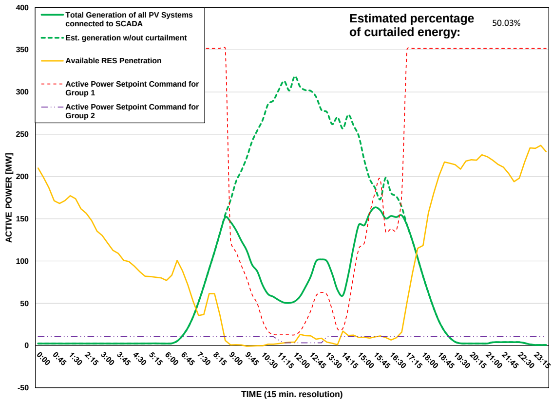
Scada PVs Generation on 16/08/2026 (curtailment time: 08:45 - 17:00)
