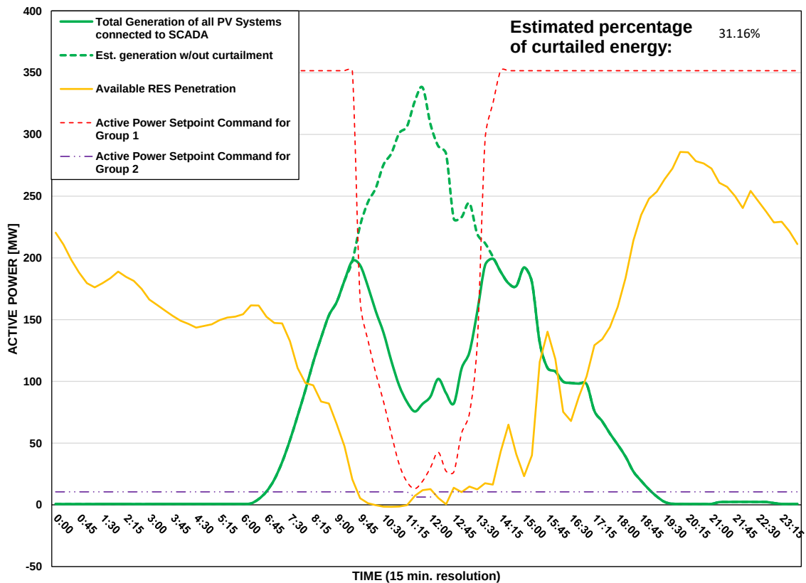
Scada PVs Generation on 17/08/2026 (curtailment time: 09:30 - 13:45)
