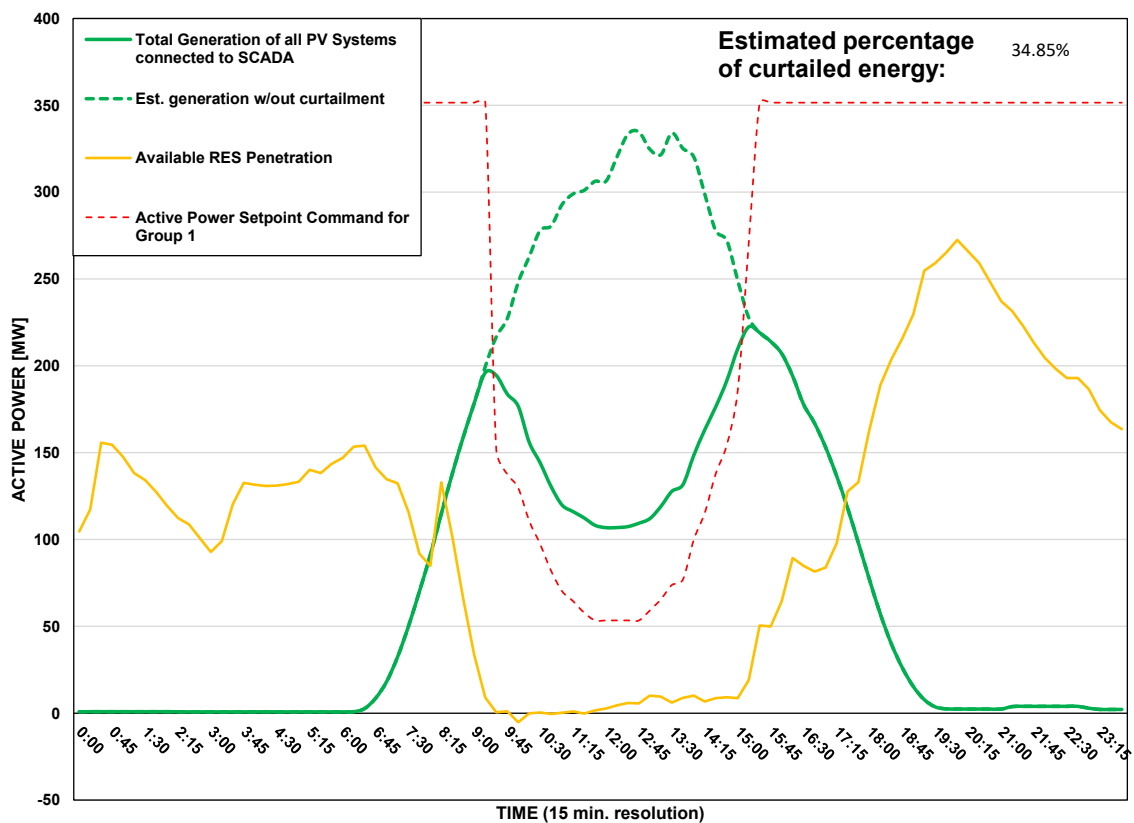
Scada PVs Generation on 19/08/2026 (curtailment time: 09:15 - 15:15)
