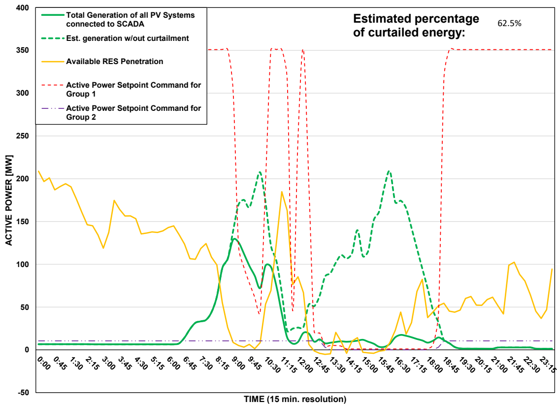
Scada PVs Generation on 29/08/2026 (curtailment time: 09:00 - 18:30)
