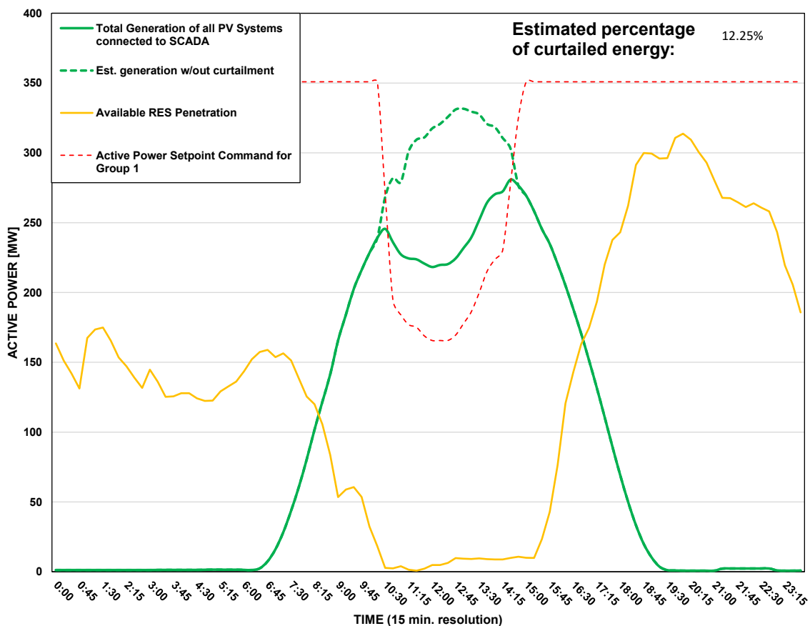
Scada PVs Generation on 24/08/2026 (curtailment time: 10:30 - 14:30)
