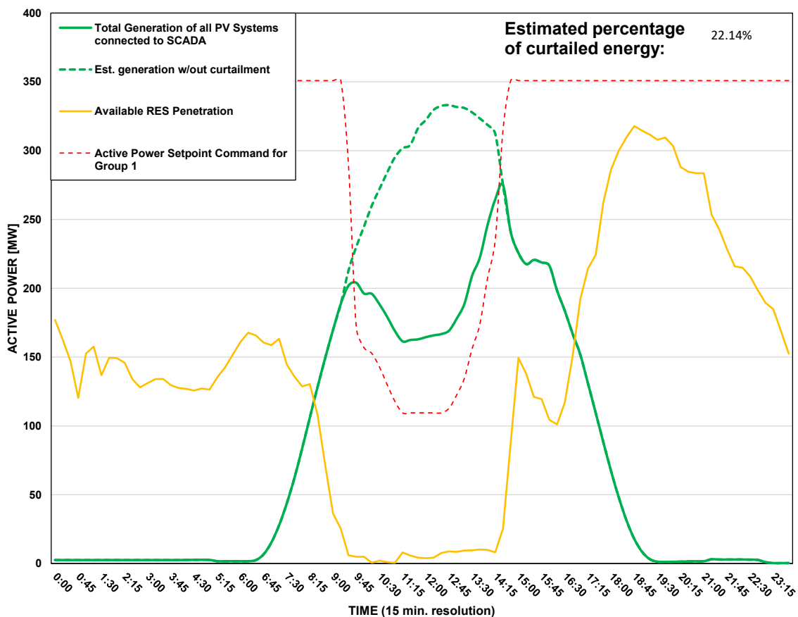
Scada PVs Generation on 27/08/2026 (curtailment time: 09:30 - 14:15)
