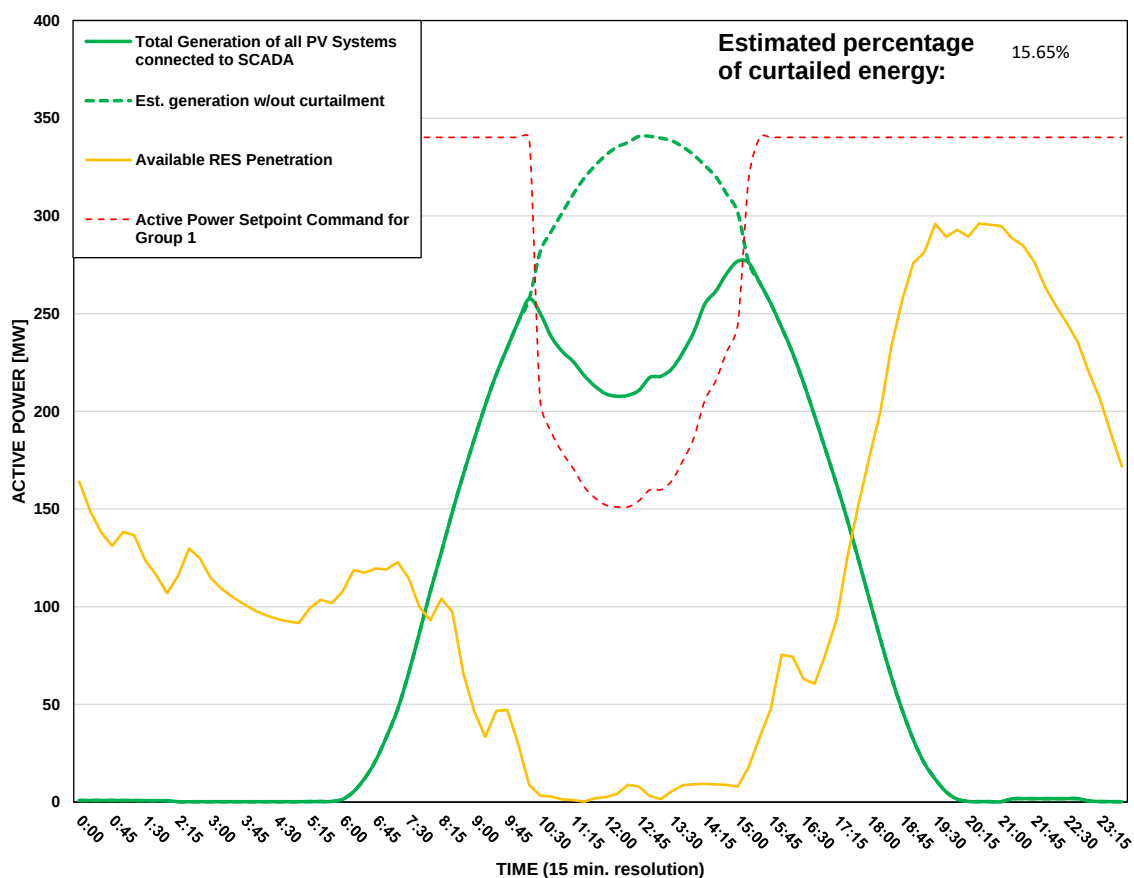
Scada PVs Generation on 13/07/2026 (curtailment time: 10:30 - 15:00)
