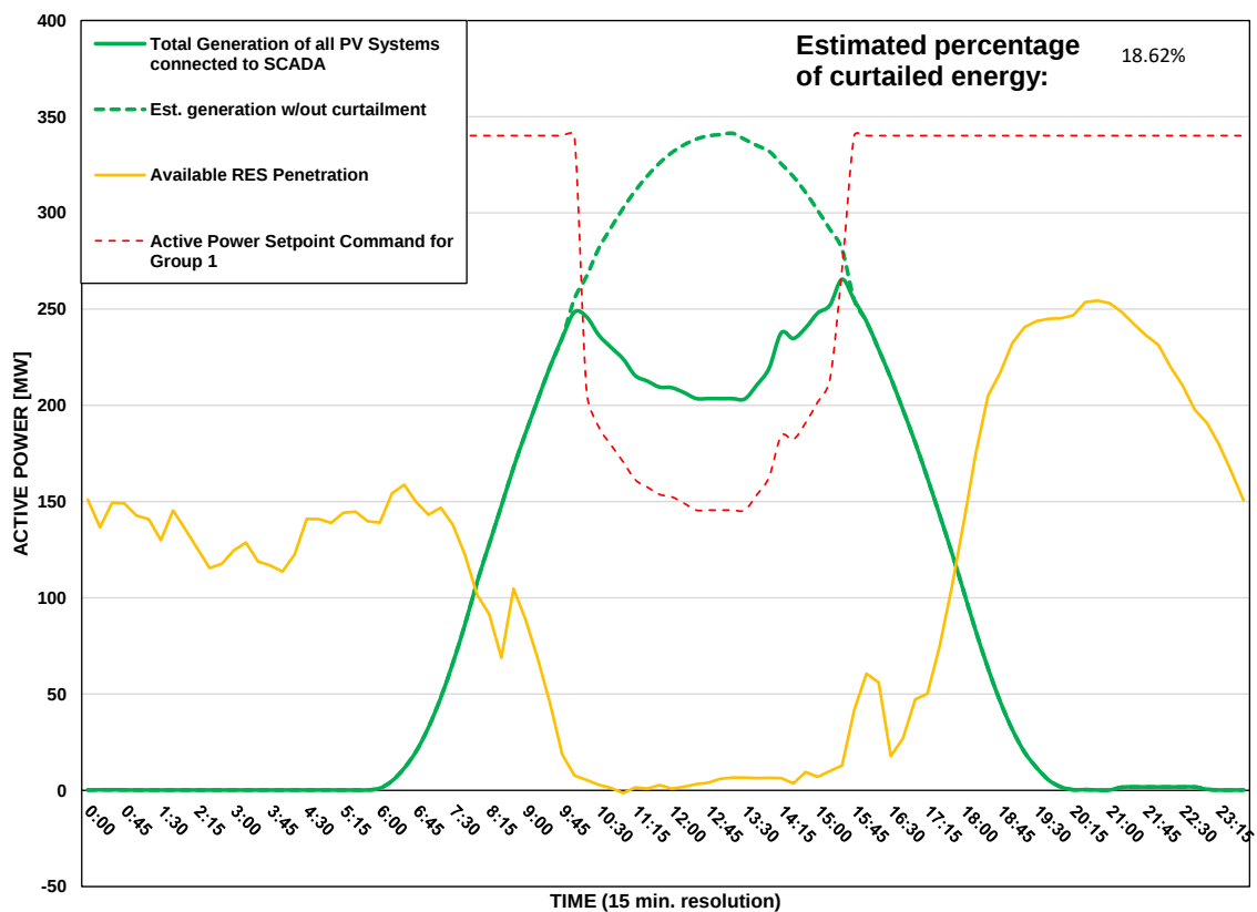
Scada PVs Generation on 14/07/2026 (curtailment time: 10:00 - 15:30)
