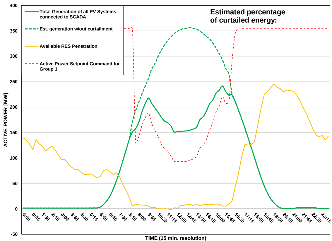
Scada PVs Generation on 02/07/2026 (curtailment time: 08:30 - 16:00)
