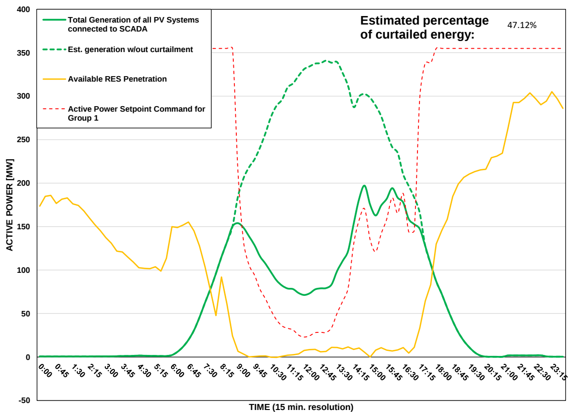
Scada PVs Generation on 05/07/2026 (curtailment time: 09:00 - 17:15)
