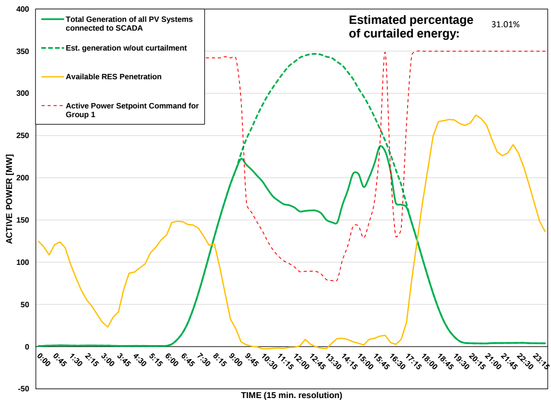
Scada PVs Generation on 27/07/2026 (curtailment time: 09:30 - 17:15)
