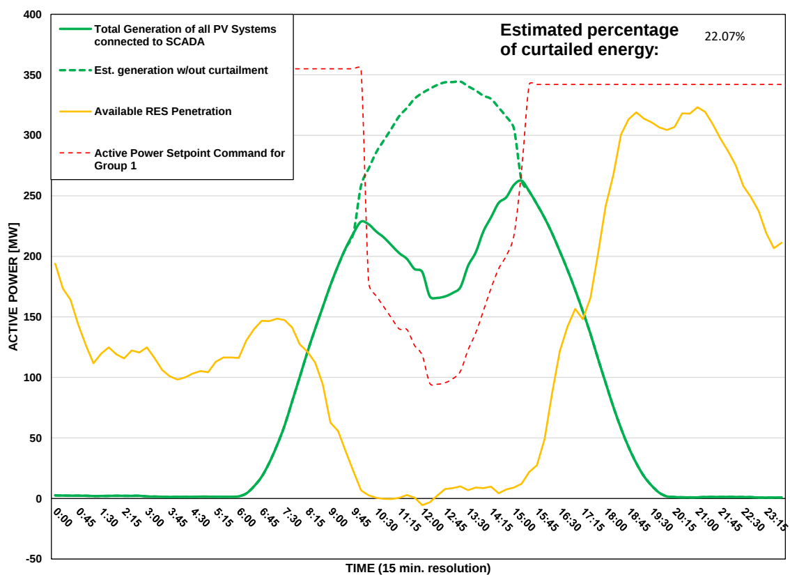
Scada PVs Generation on 23/07/2026 (curtailment time: 10:00 - 15:00)
