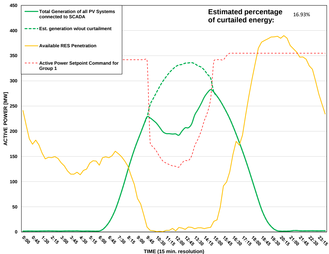
Scada PVs Generation on 22/07/2026 (curtailment time: 10:00 - 14:45)
