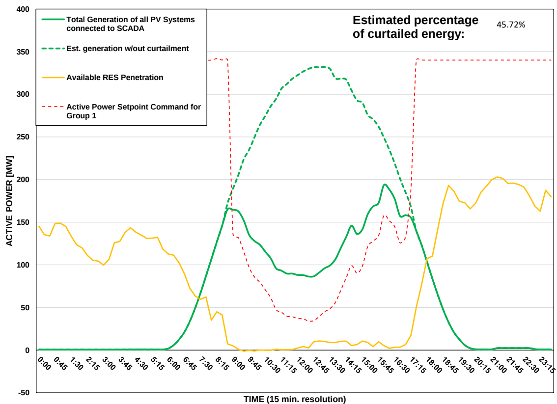
Scada PVs Generation on 12/07/2026 (curtailment time: 08:45 - 17:15)
