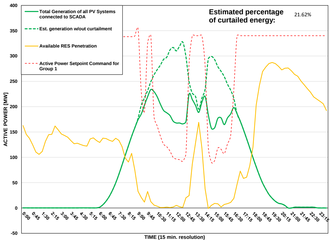
Scada PVs Generation on 07/07/2026 (curtailment time: 09:15 - 16:30)
