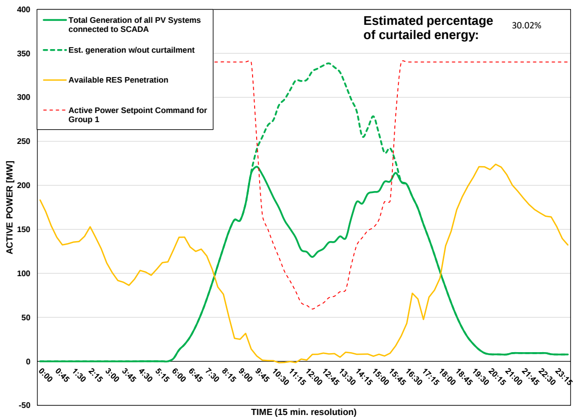
Scada PVs Generation on 08/07/2026 (curtailment time: 09:45 - 16:00)
