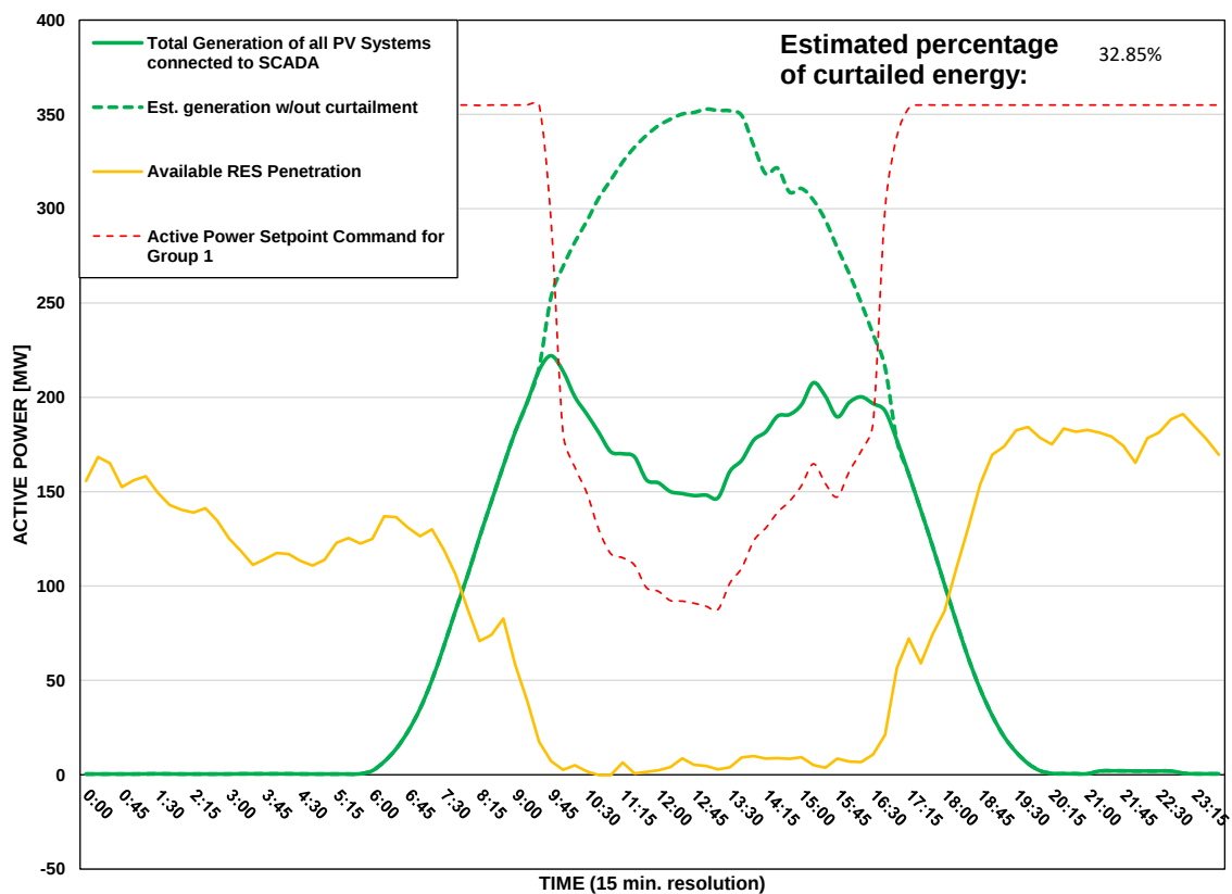
Scada PVs Generation on 03/07/2026 (curtailment time: 09:45 - 16:45)
