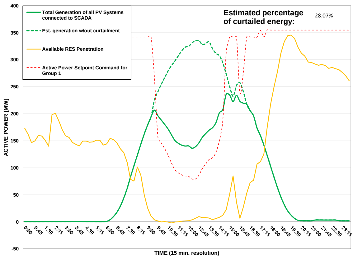
Scada PVs Generation on 18/07/2026 (curtailment time: 09:30 - 16:00)
