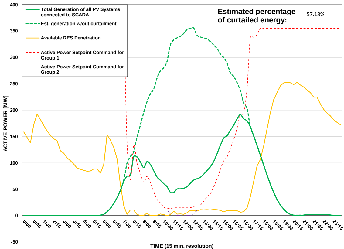
Scada PVs Generation on 04/07/2026 (curtailment time: 07:45 - 16:45)
