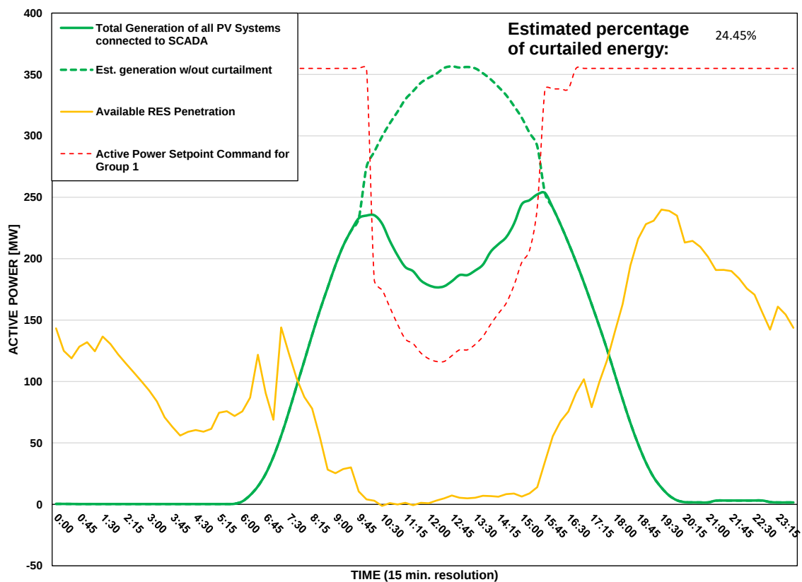
Scada PVs Generation on 01/07/2026 (curtailment time: 10:00 - 15:30)
