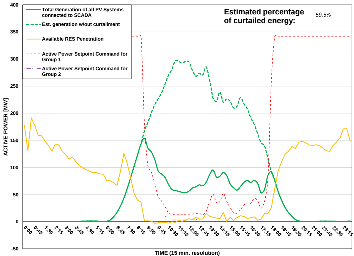
Scada PVs Generation on 25/07/2026 (curtailment time: 08:45 - 17:45)
