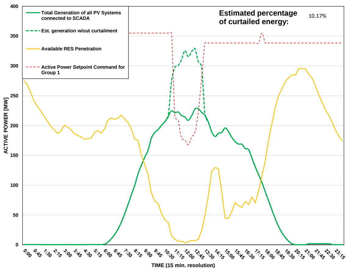
Scada PVs Generation on 06/07/2026 (curtailment time: 11:00 - 13:15)
