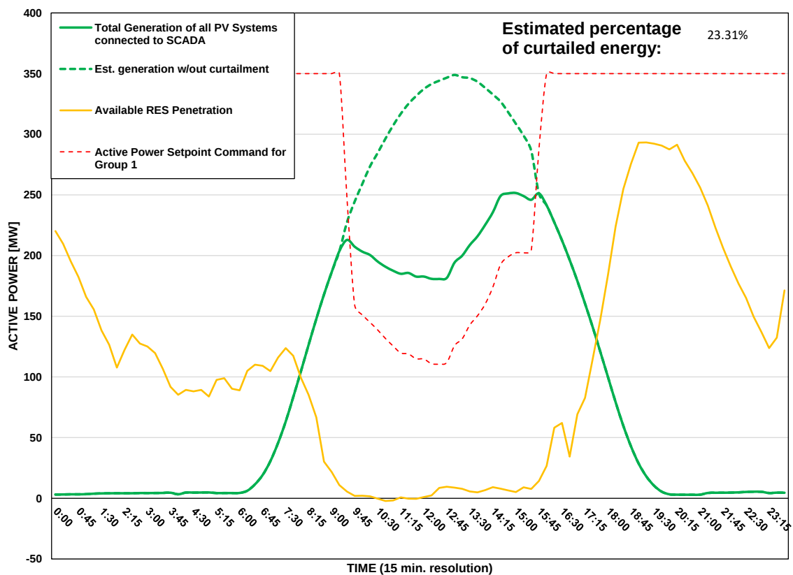
Scada PVs Generation on 29/07/2026 (curtailment time: 09:30 - 15:30)
