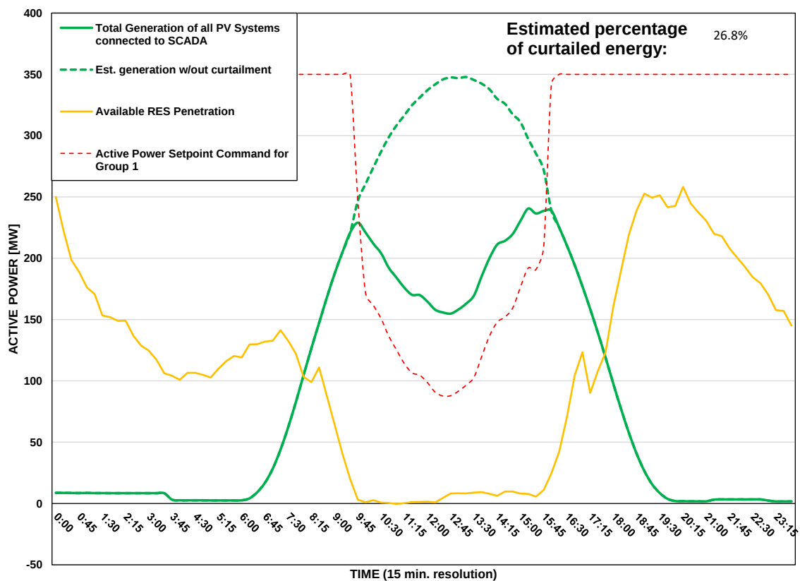
Scada PVs Generation on 31/07/2026 (curtailment time: 09:45 - 15:45)
