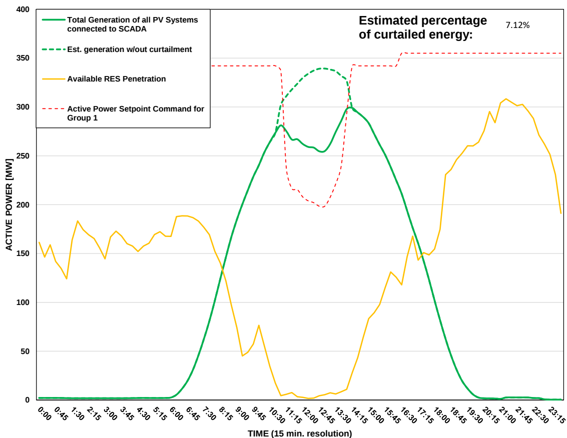
Scada PVs Generation on 20/07/2026 (curtailment time: 11:00 - 14:00)
