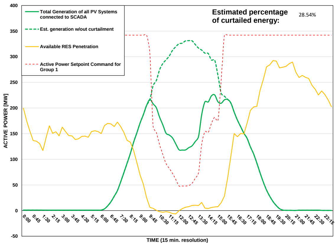
Scada PVs Generation on 24/07/2026 (curtailment time: 10:00 - 15:30)
