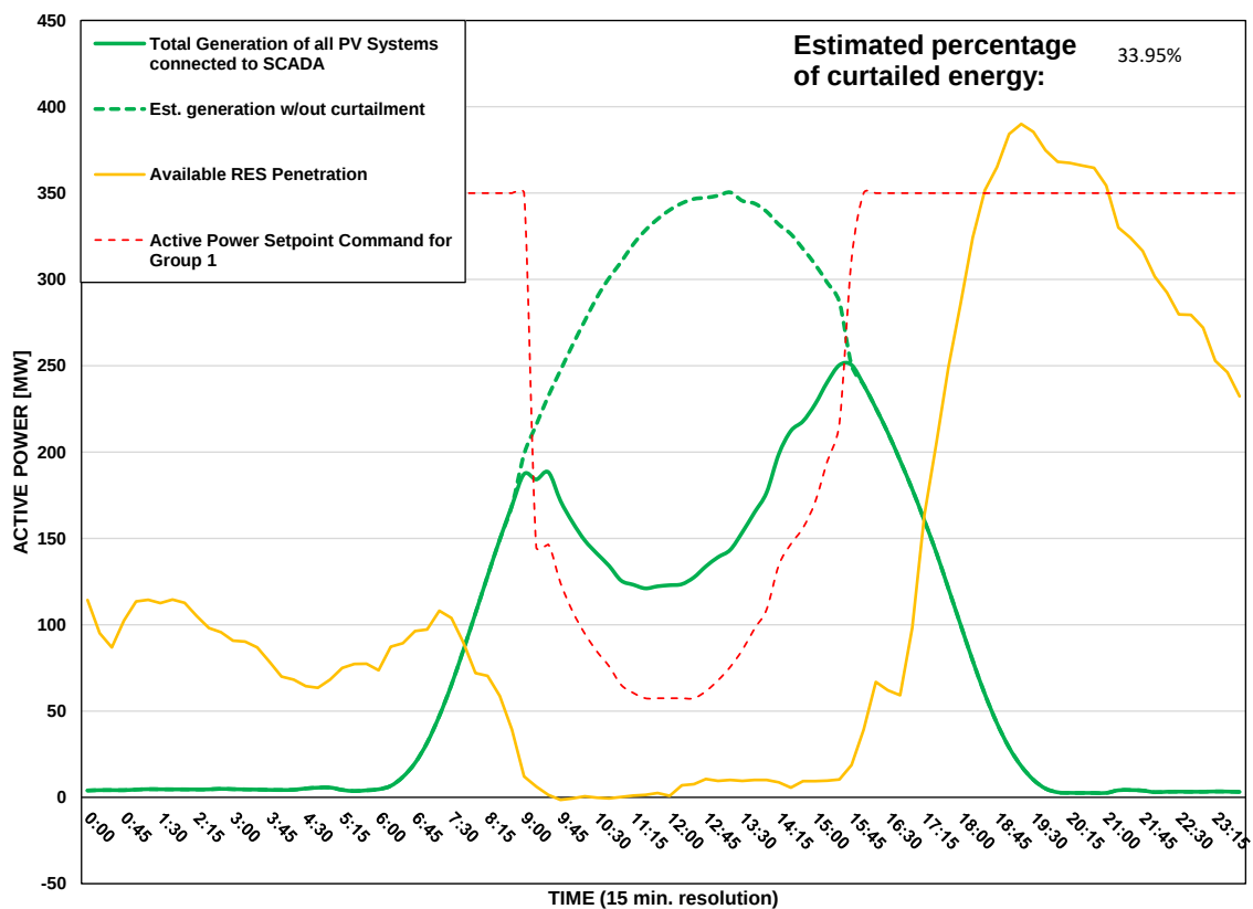
Scada PVs Generation on 28/07/2026 (curtailment time: 09:00 - 15:30)
