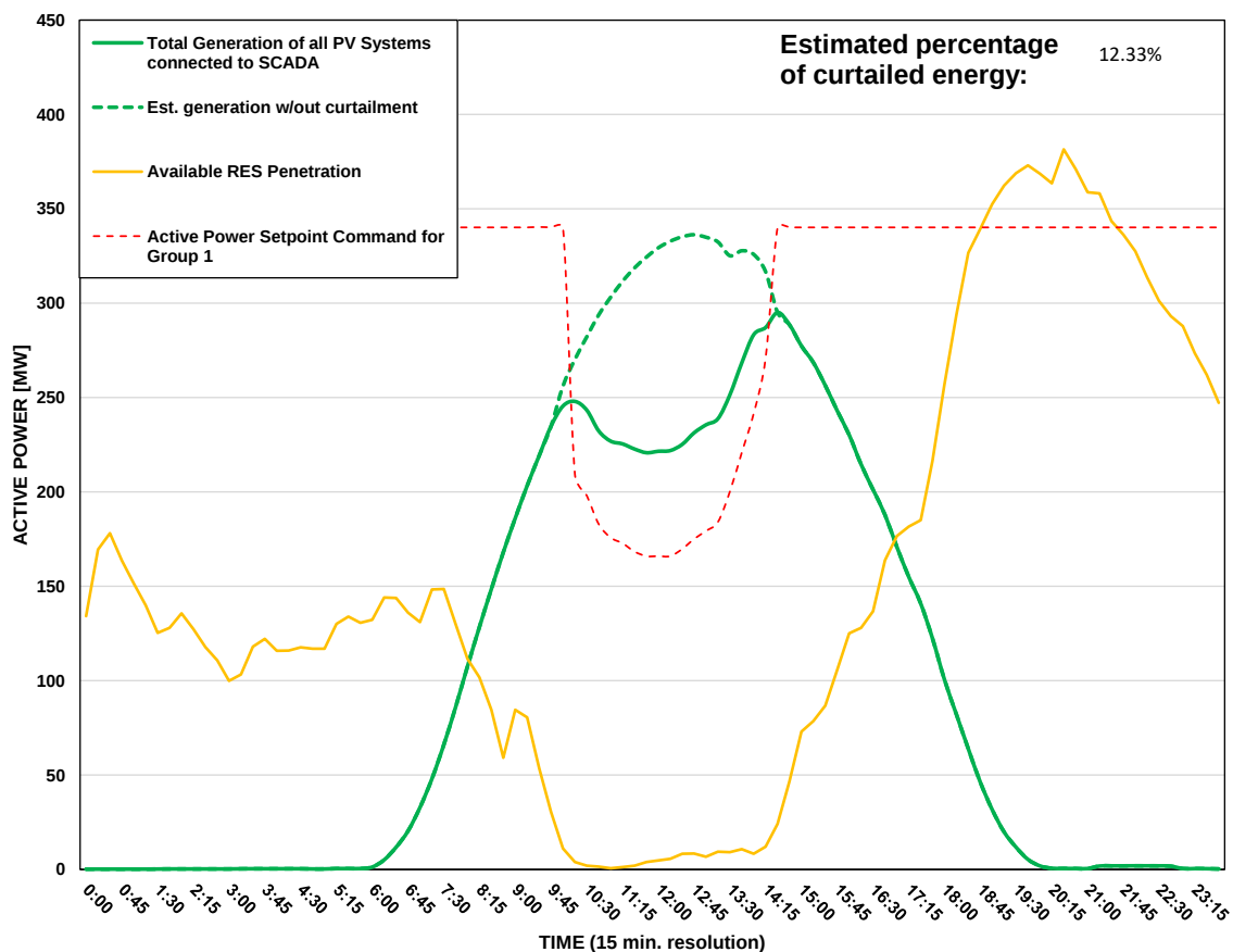
Scada PVs Generation on 15/07/2026 (curtailment time: 10:00 - 14:15)
