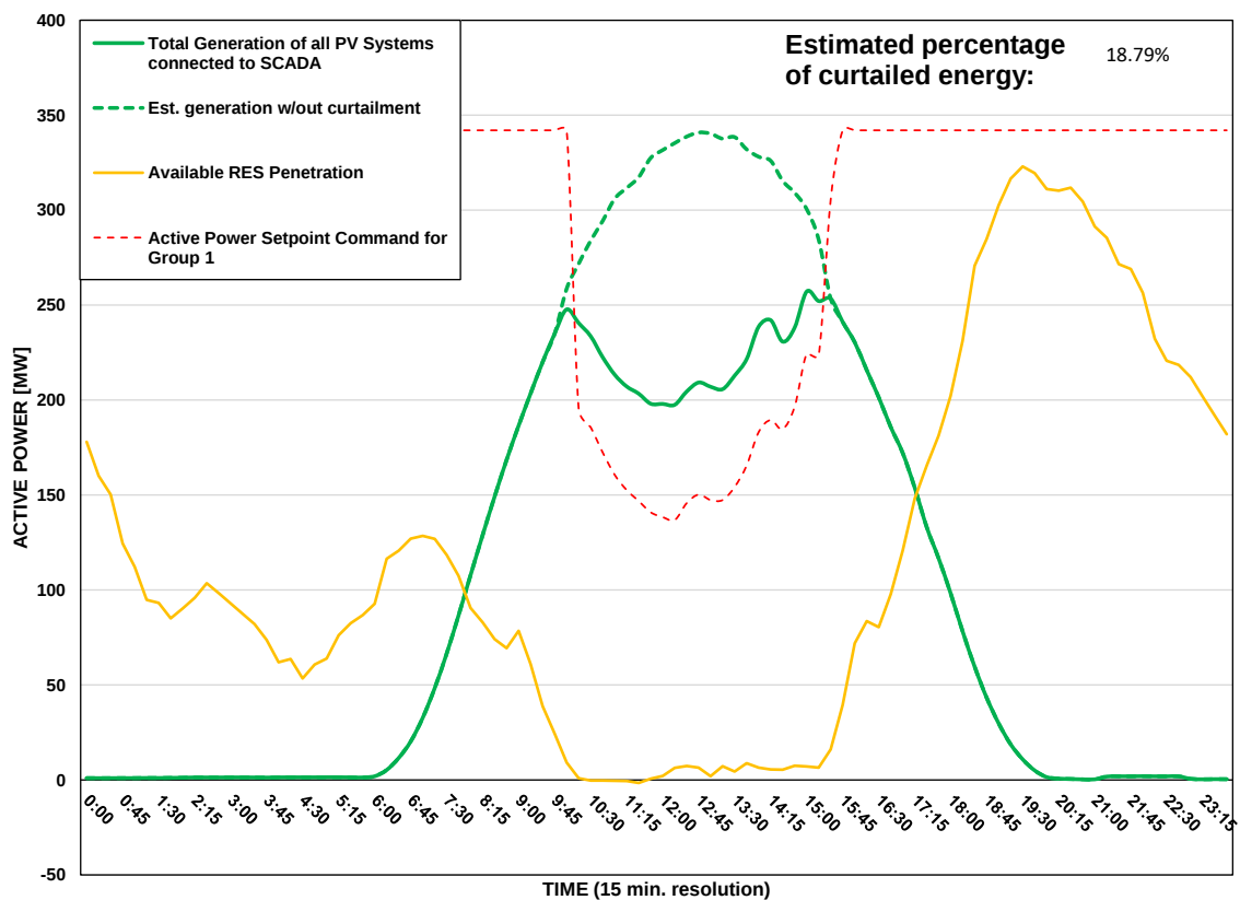
Scada PVs Generation on 17/07/2026 (curtailment time: 10:00 - 15:15)
