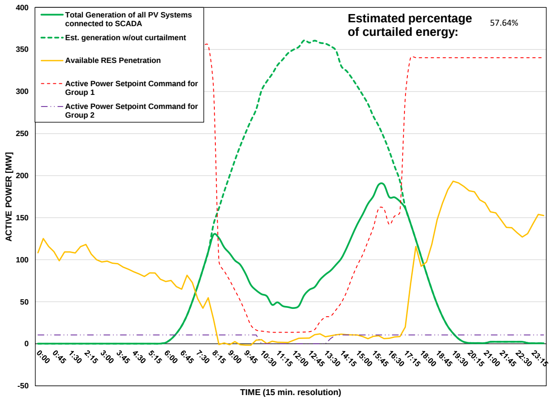
Scada PVs Generation on 11/07/2026 (curtailment time: 08:15 - 17:00)
