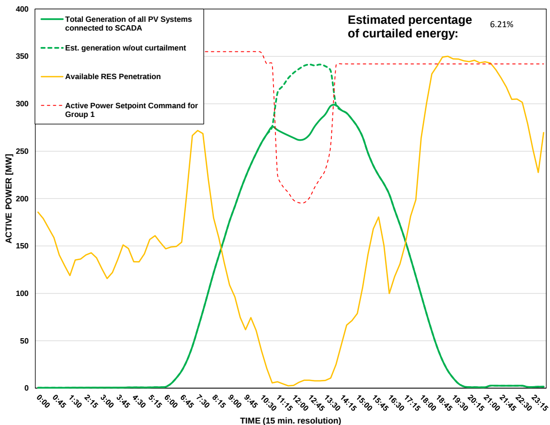
Scada PVs Generation on 21/07/2026 (curtailment time: 11:15 - 13:45)
