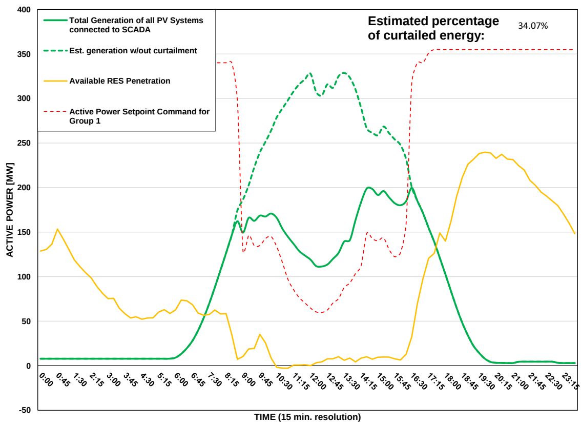
Scada PVs Generation on 09/07/2026 (curtailment time: 08:45 - 16:15)
