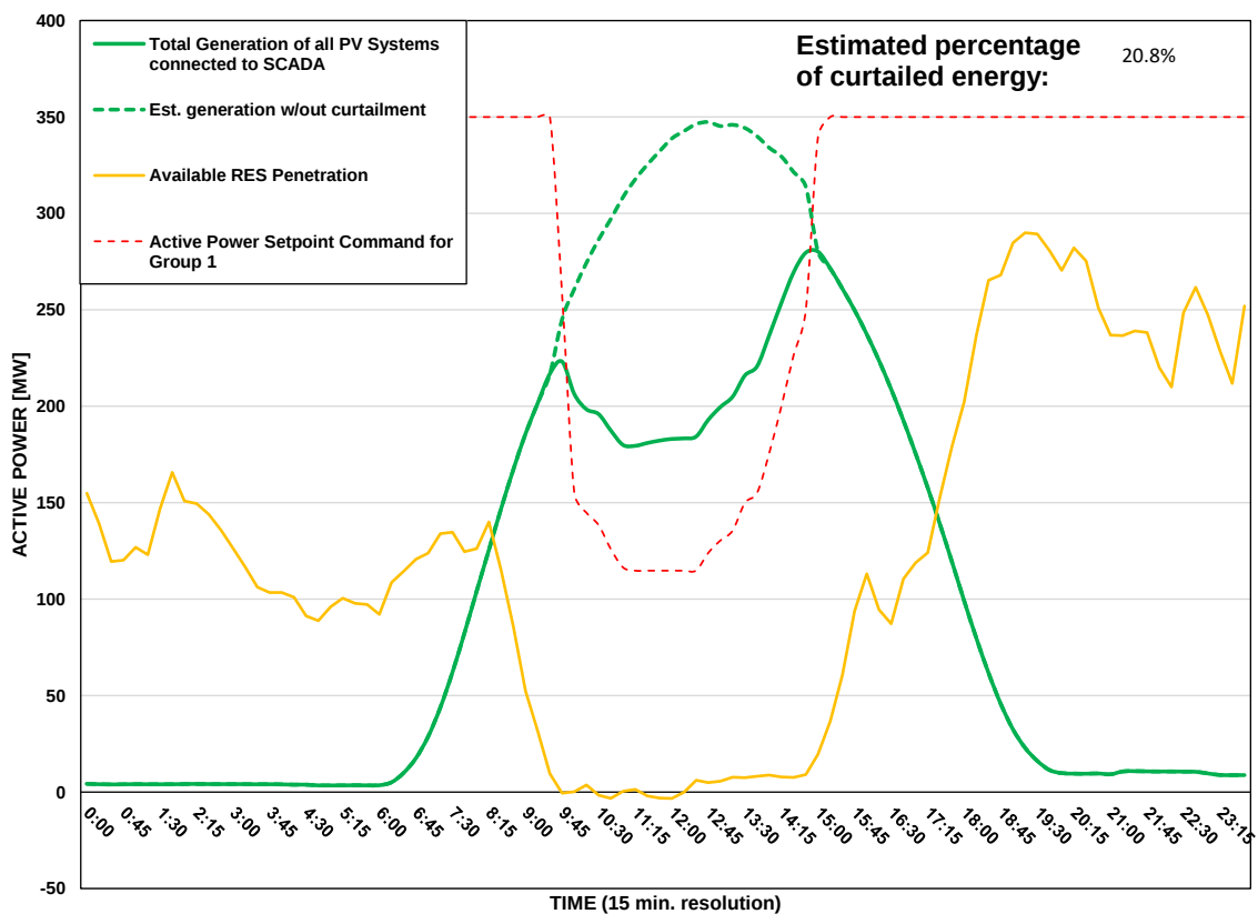
Scada PVs Generation on 30/07/2026 (curtailment time: 09:45 - 14:45)
