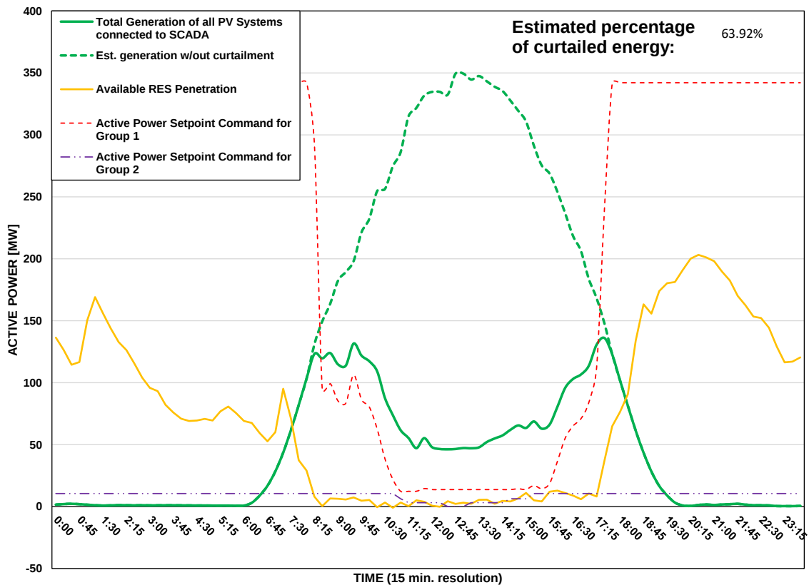
Scada PVs Generation on 26/07/2026 (curtailment time: 08:15 - 17:30)
