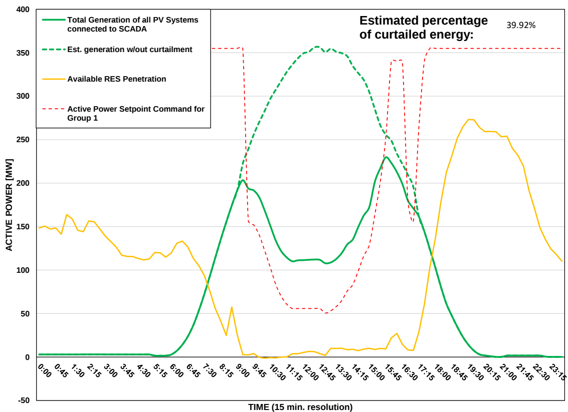
Scada PVs Generation on 10/07/2026 (curtailment time: 09:15 - 17:00)
