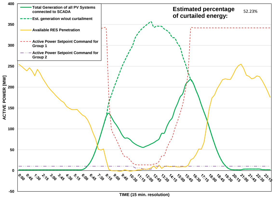
Scada PVs Generation on 19/07/2026 (curtailment time: 08:30 - 16:00)
