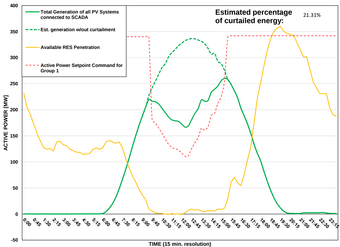
Scada PVs Generation on 16/07/2026 (curtailment time: 09:30 - 15:15)
